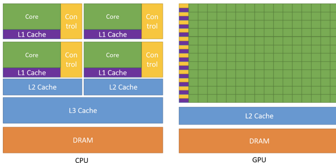
Figure 4: Architectural design of a typical CPU compared to a typical GPU. Source: CUDA documentation, Nvidia Corporation https://docs.nvidia.com/cuda/cuda-c-programming-guide/
