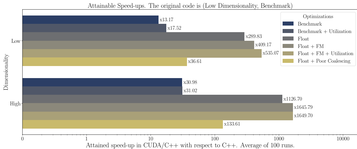
Figure D.10: Attainable speed-ups in the original Fernández-Villaverde and Valencia (2018)'s code, by employed optimizations and dimensionality (CUDA/C++ vs single-threaded C++).
